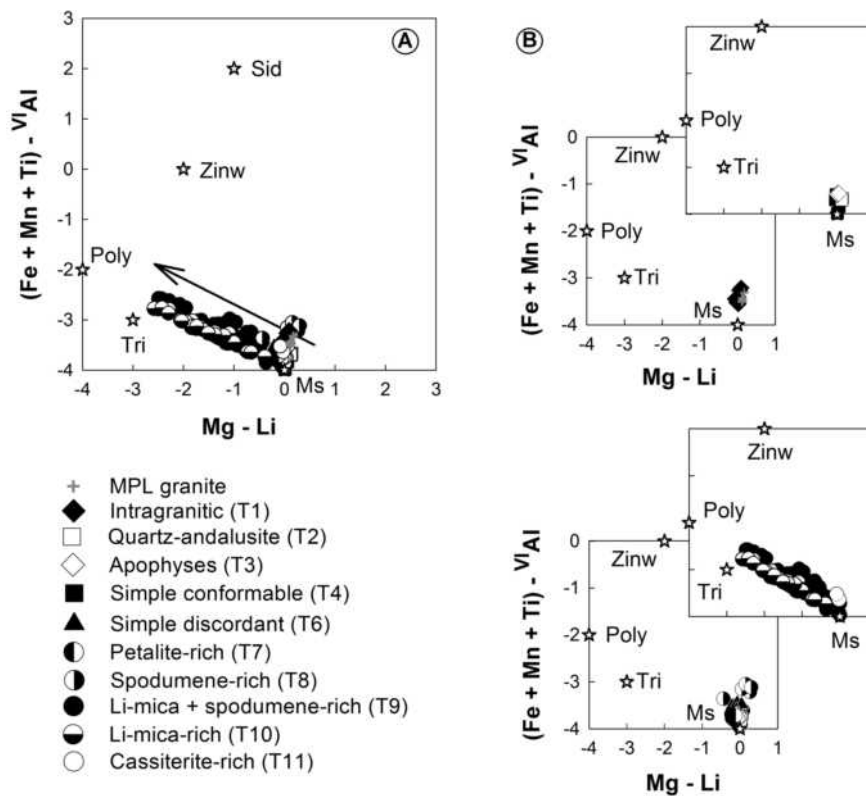
FIGURE 2. (a) Mg - Li vs. (Fe + Mn + Ti) - VAl and (b) Figure 2a inset, for the micas associated with the different pegmatite types from the Fregeneda-Almendra field. (All data in apfu.)
