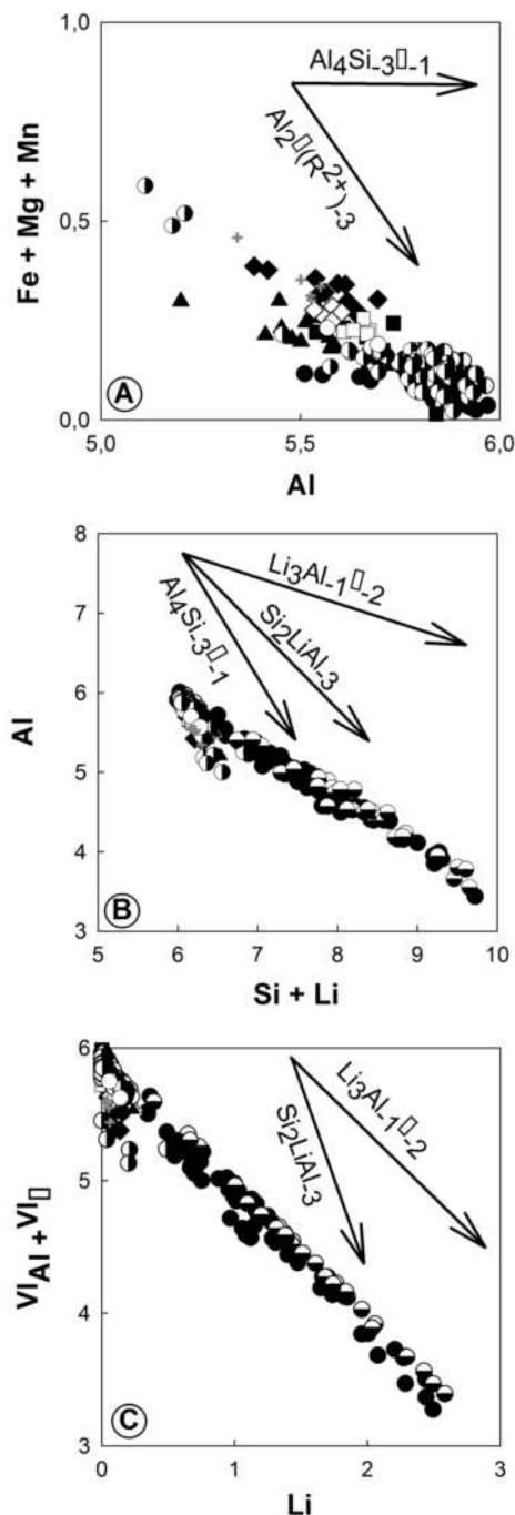
FIGURE 4. (a) Al vs. Fe + Mg + Mn (F wt% < 1), (b) Si + Li vs. Al, and (c) Li vs. VI_{Al} + VI_{\Box} , for the micas associated with the different pegmatite types from the Fregeneda-Almendra field. The arrows labeled with the exchange vectors represent the direction of the vector that reflects the evolutionary trend of the micas. (Symbols as in Fig. 2; all data in apfu; R^{2+} = Fe + Mg + Mn .)
