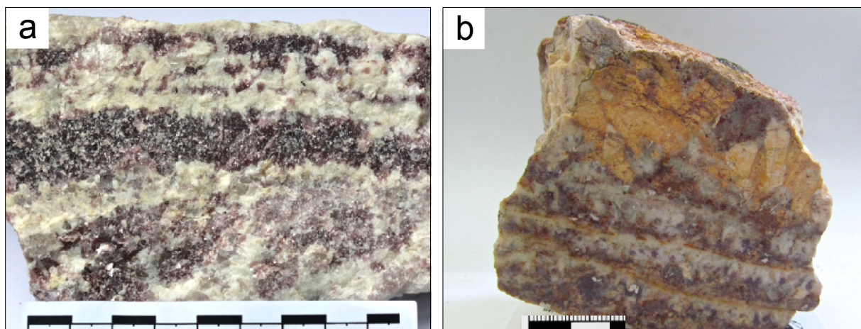
Fig. 2: (a) Rythmic layering with alternating lepidolite-rich and albite-rich bands in an aplitic-pegmatite dyke from the Gonçalves field; (b) similar texture as (a) in the lower part, plus some wedge-shaped crystals of K-feldspar in the upper part, from the stockscheider of Castillejo de Dos Casas (Roda-Robles et al., 2016).
