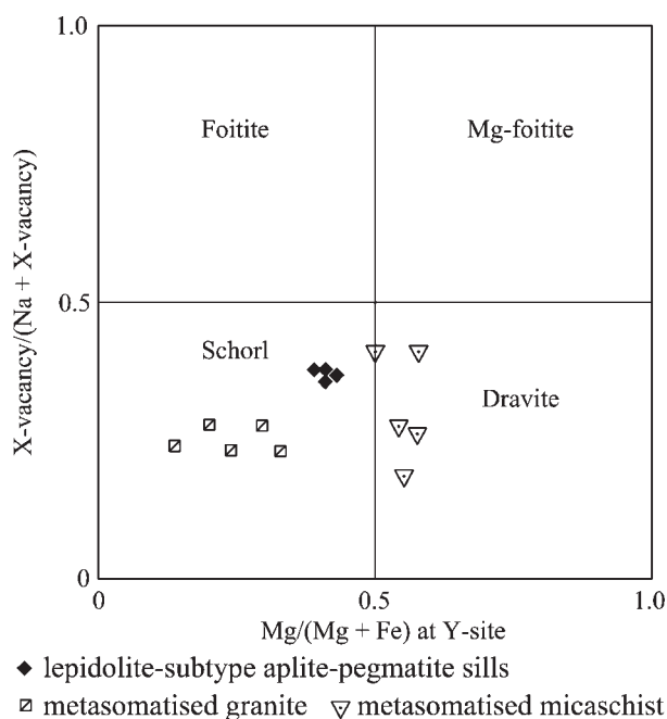
Fig. 11. Tourmaline compositions from lepidolite-subtype aplite-pegmatite sills from Gonalo and adjacent granite and micaschist. Schorl from sills has a composition distinct from metasomatic schorl of granite and metasomatic dravite of micaschist.
