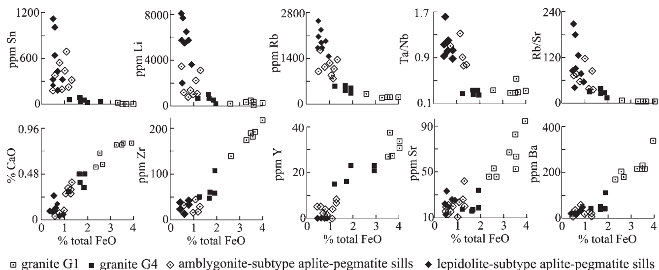
Fig. 6. Selected variation diagrams of granites G1 and G4 from Guarda-Belmonte and granitic aplite-pegmatite sills from Gonçalves, suggesting that aplite-pegmatite sills are not related to this series G1–G4.
