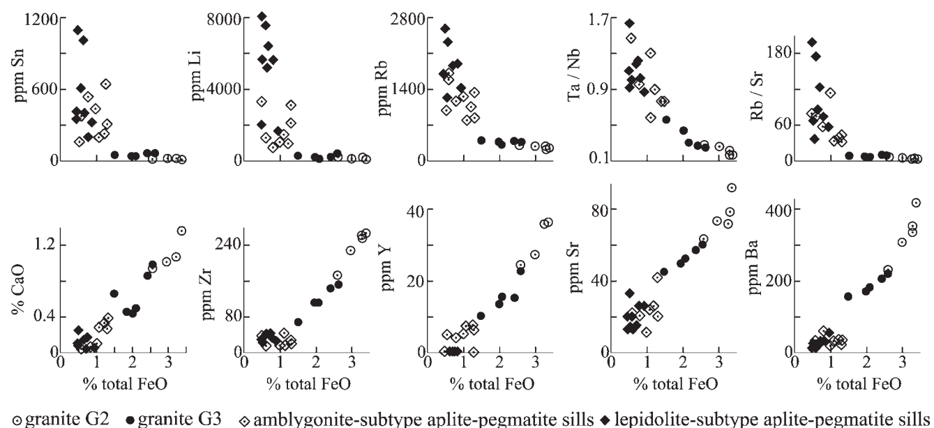
Fig. 7. Variation diagrams of granites G2 and G3 from Guarda-Belmonte and granitic aplite-pegmatite sills from Gonçalves, suggesting a crystal fractionation model.
