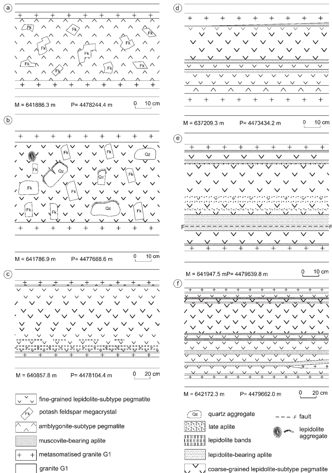
Fig. 3. Sketches of aplite-pegmatite sills from Gonçalo (Guarda). (a–f) From the simplest to those containing up to 14–15 layers.
