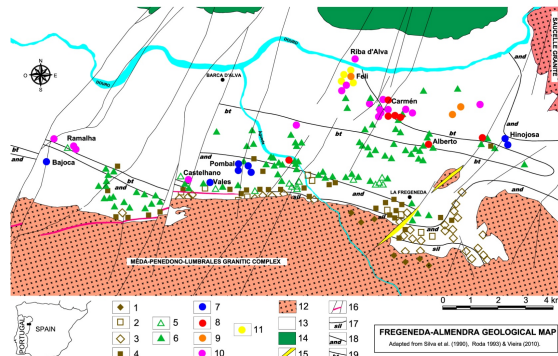
FIGURE 1. Distribution of the pegmatite types in the Fregeneda-Almendra area.
