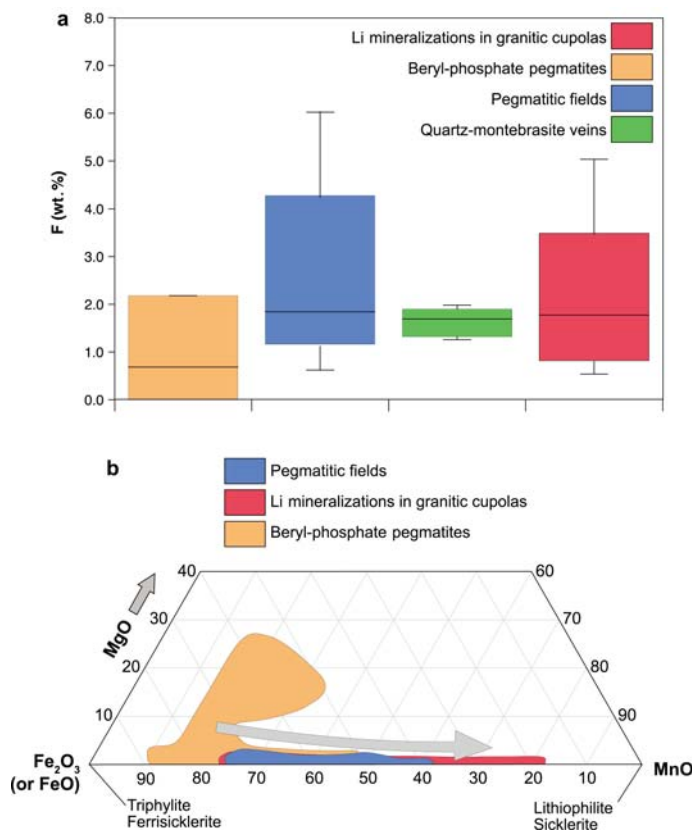
FIG. 5. (a) Variation in the F-content for members of the amblygonite–montebbrasite series associated with the different types of Li mineralization; and (b) ternary plot of the Fe 2 O 3 –MnO–MgO contents for the Li–Fe–Mn phosphates from the different types of Li mineralization.
