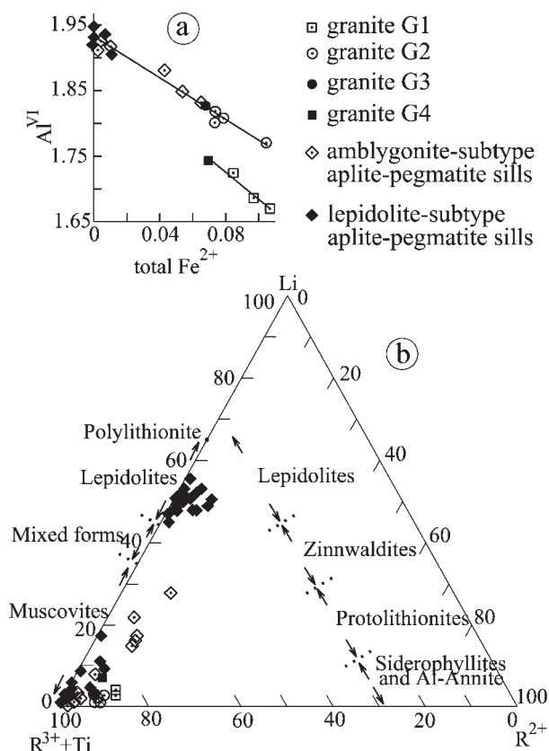
Fig. 10. Crystal chemistry of micas from granites from Guarda-Belmonte and granitic aplite-pegmatite sills from Gonalo. (a) Al^{VI} vs. Fe diagram showing two trends for magmatic muscovites, one for G1 and G4 and another for G2, G3 and sills; (b) octahedral cation plot for micas from these granitic rocks, according to the classification of Foster (1960); however, zinnwaldite is a series name for trioctahedral mica on, or close to, the siderophyllite-polyolithionite join (Rieder et al. , 1999); R^{3+} = Al^{VI} , R^{2+} = (Fe_t^{2+} + Mn^{2+} + Mg) .
