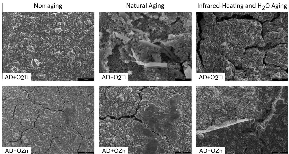
Fig. 3. SEM images corresponding to textural variations of binder samples with poppyseed oil (AD) and titanium white ( O_2Ti ) and zinc white (OZn), respectively. The images show non-aged pictorial films, naturally aged ones and those aged by warming and saturated relative humidity. From left to right appears a less smooth textural variation, as well as the appearance of scattered binders in the form of fine threads and an increase in cracks and microfissures. The textural changes provoked visual variations in total colour ( \Delta E ), loss of luminosity ( \Delta L ), and loss of chroma ( \Delta C ), with the appearance of yellowing in the samples.
