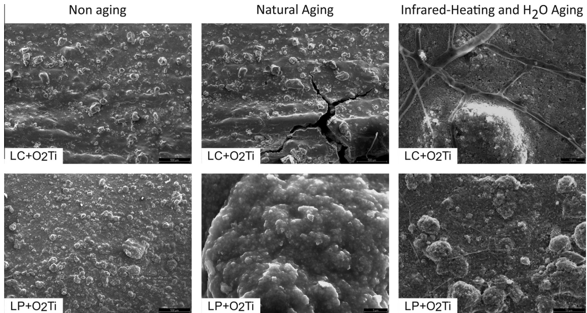
Fig. 2. SEM images corresponding to textural variations in samples of binders with raw linseed oil (LC) and polymerized linseed oil (LP) and titanium white ( O_2Ti ), not aged, naturally aged, and aged by heating and saturated relative humidity. From left to right appears less smooth textural variation, as well as the appearance of scattered binders in the form of fine threads. All of these changes provoked visual variations in total colour ( \Delta E ), loss in luminosity ( \Delta L ) and in chroma ( \Delta C ), with the appearance of yellowing in the samples.
