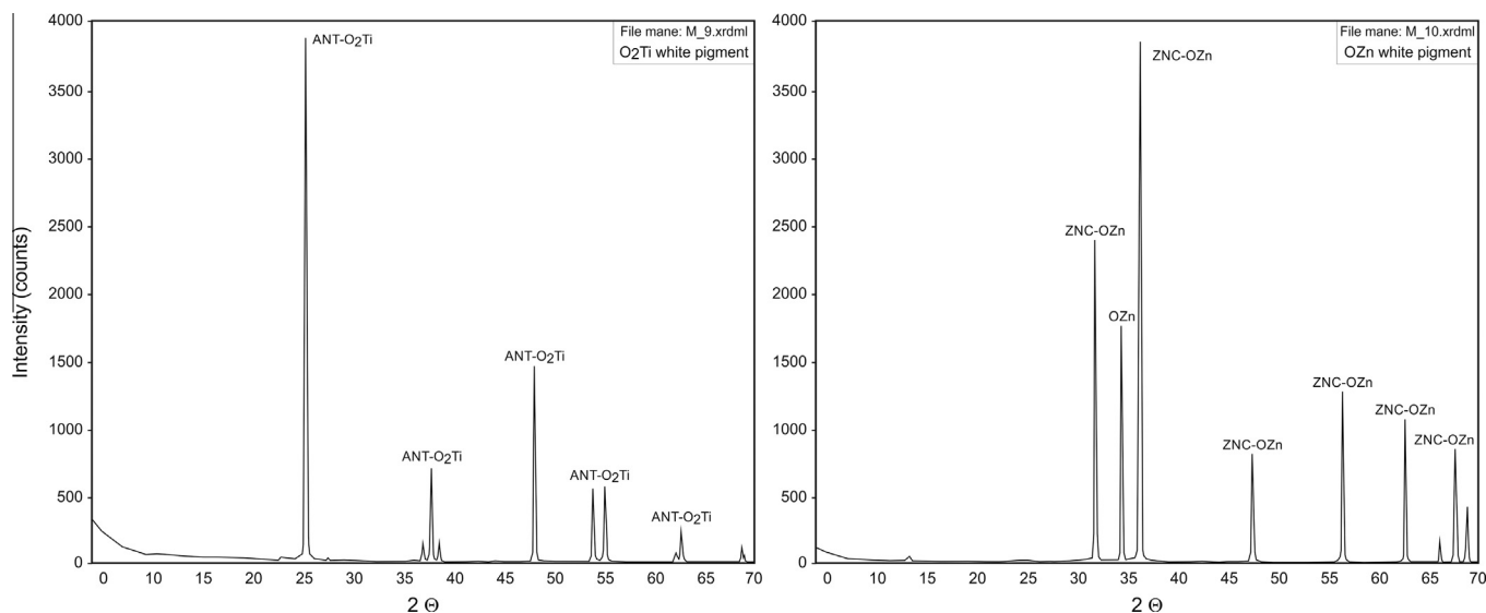
Fig. 1. XRD diffractograms of the pigments studied: O 2 Ti white pigment and OZn white pigment.
