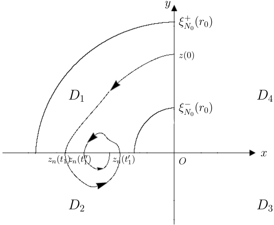
Figure 2: A solution turning back to region D_1 .
