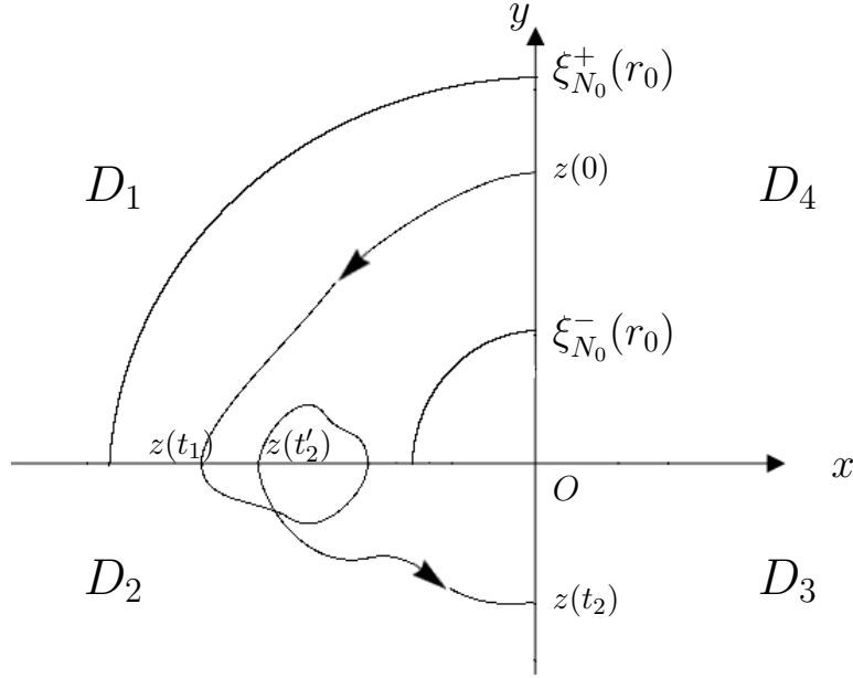
Figure 1: The spiral property
