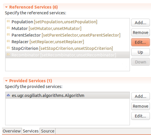
Figure 6.8 Graphic user in- terface in Eclipse that generates the Service Descriptor of Figure 6.7
