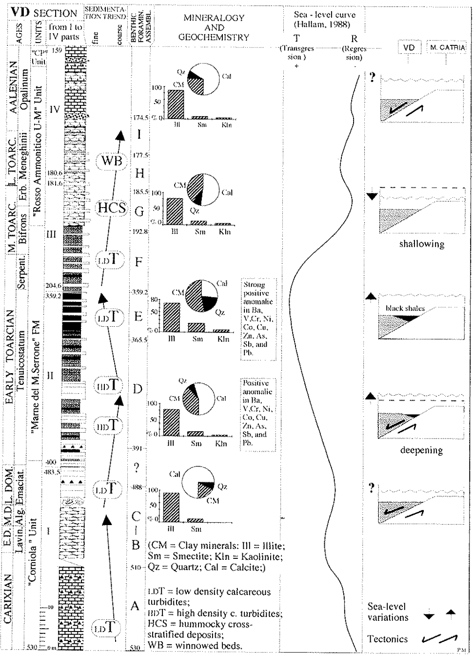
Fig. 21. Valdorbia Section related to the Hallam (1988) eustatic curve. Tectonic and eustacy interpretations have been reported on the right side, according to depositional trends, mineralogy and geochemistry.
