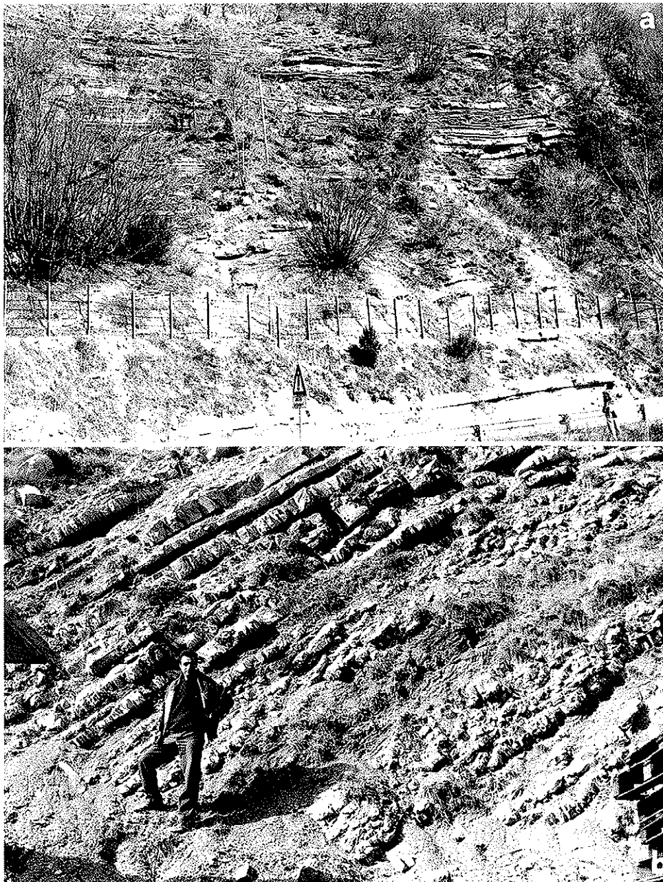
Fig. 3. a The MS-RAUM transition (Middle-Upper Toarcian). The MS Formation consists of soft grey marl intercalated with calcarenitic-calcsiltitic turbidites. The RAUM Unit is represented by reddish nodular marl, limestones and reddish nodular marls. Sharp-based hummocky cross-stratified calcarenites (HCS) occur in this part of the VD Section. b Black shale deposits with low-density calcsiltitic turbidites containing radiolarian (Lower Toarcian, middle-upper part of Tenuicostatum Zone).
