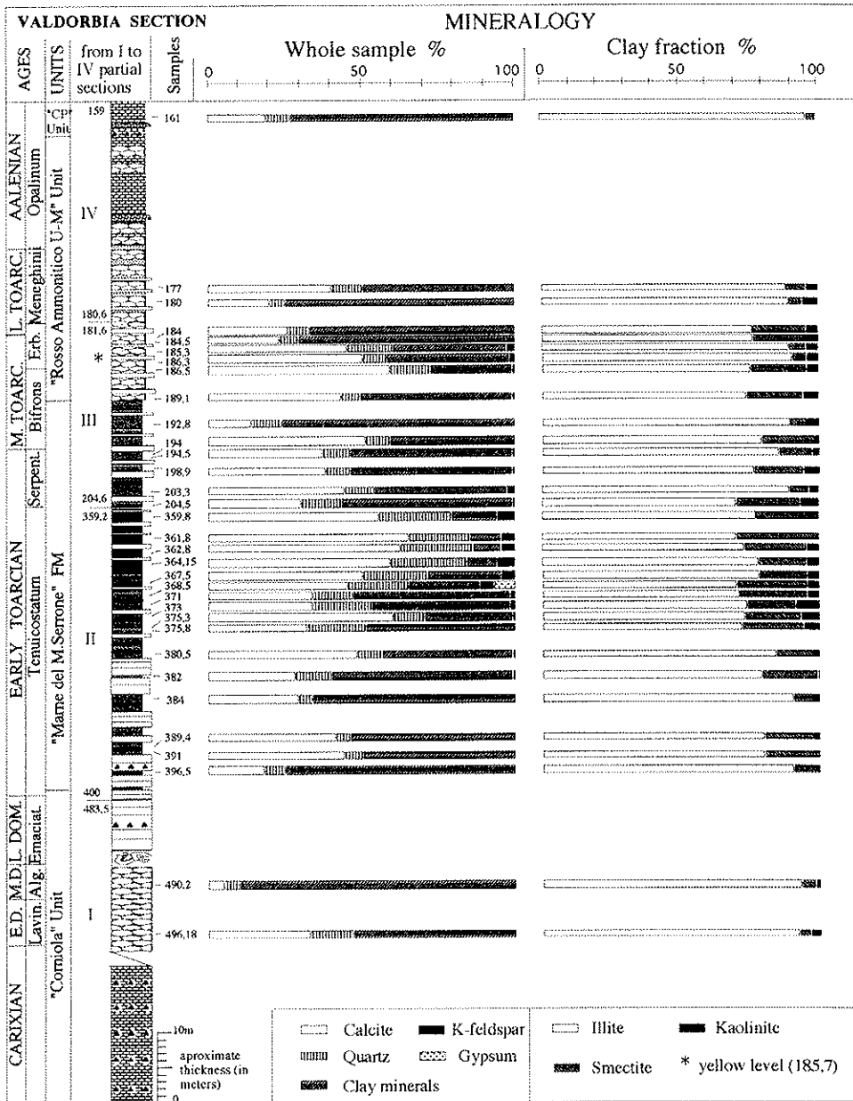
Fig. 19. Mineralogy of the studied samples.
