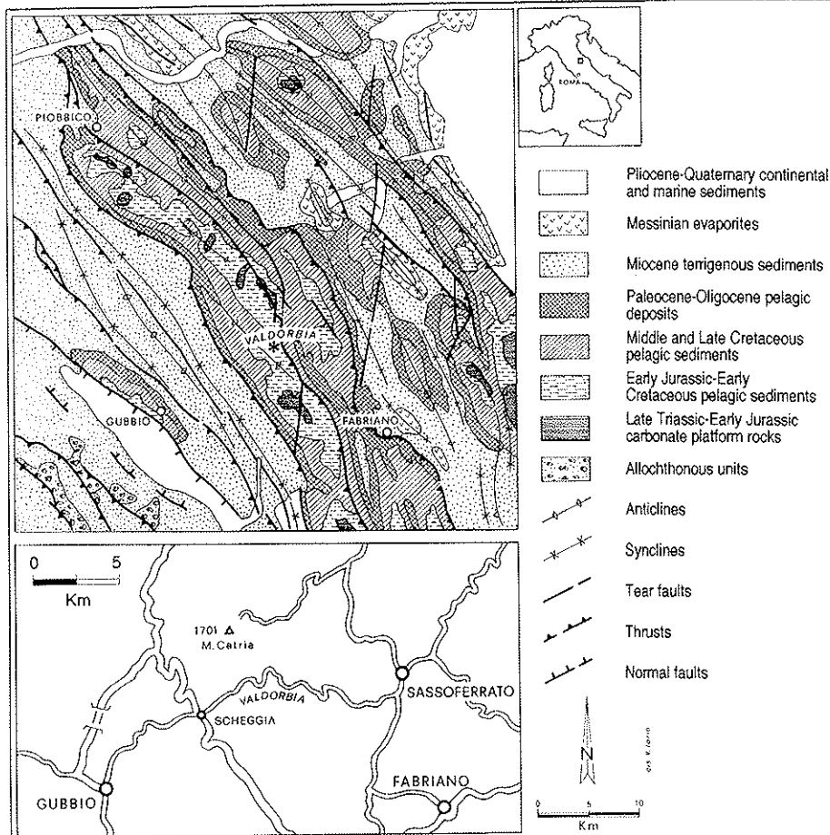
Fig. 1. Schematic geological map and location of the Valdorbria Section.
