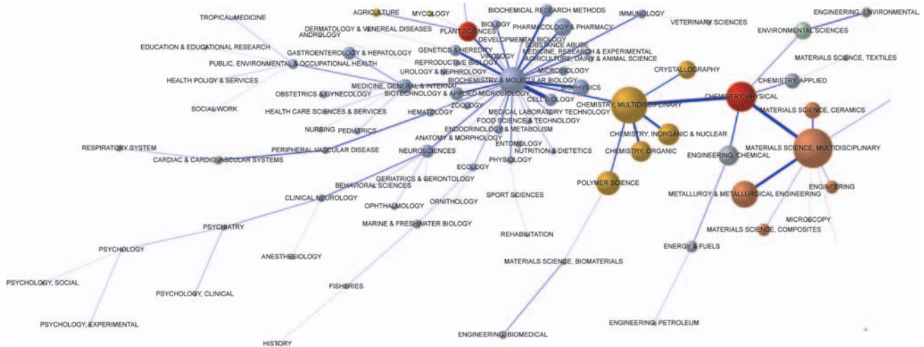
Figure 4: Enlargement of the center of the Chinese Domain 2002.
