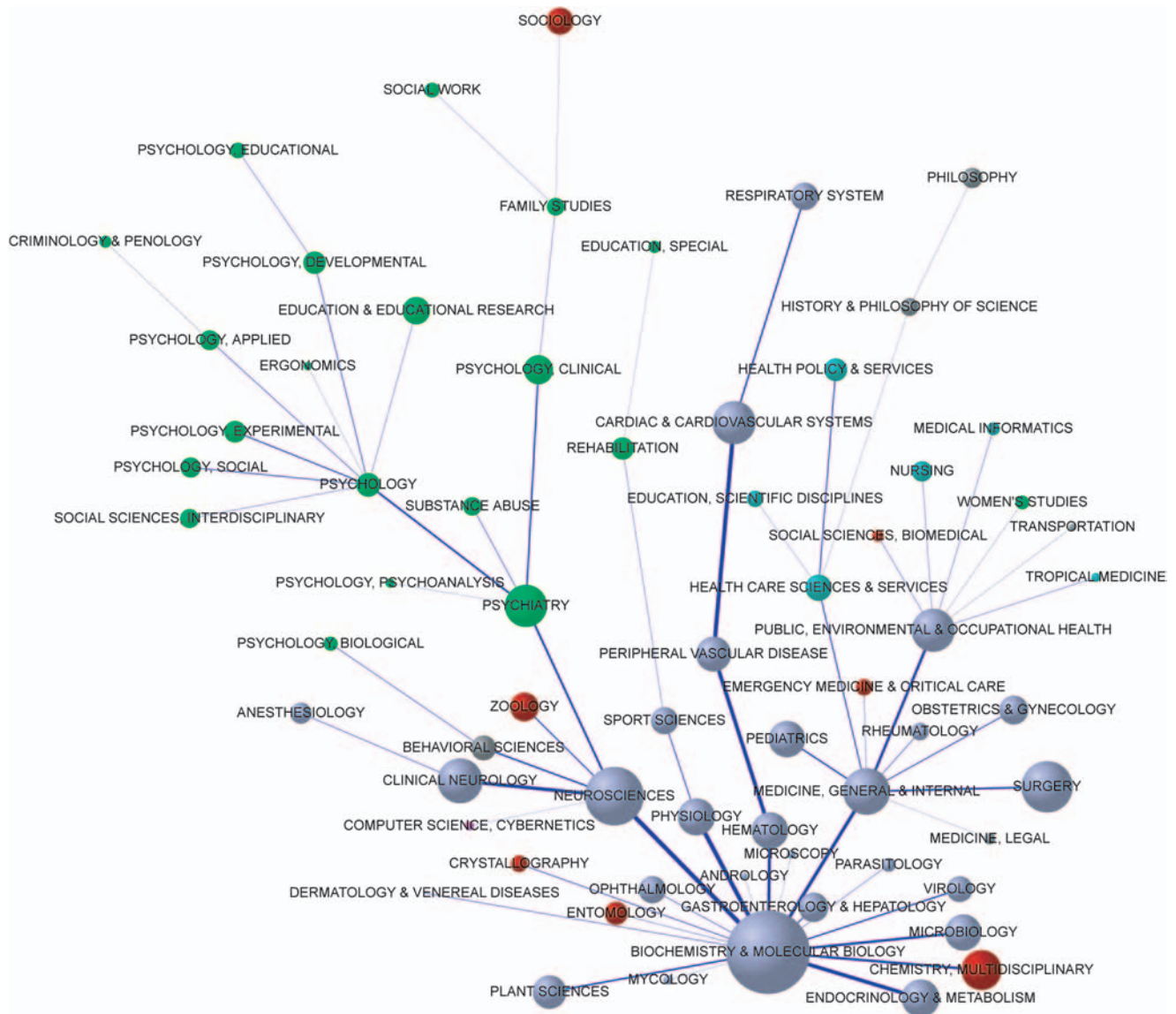
Figure 3: Enlargement of the center of the US Domain 2002.
