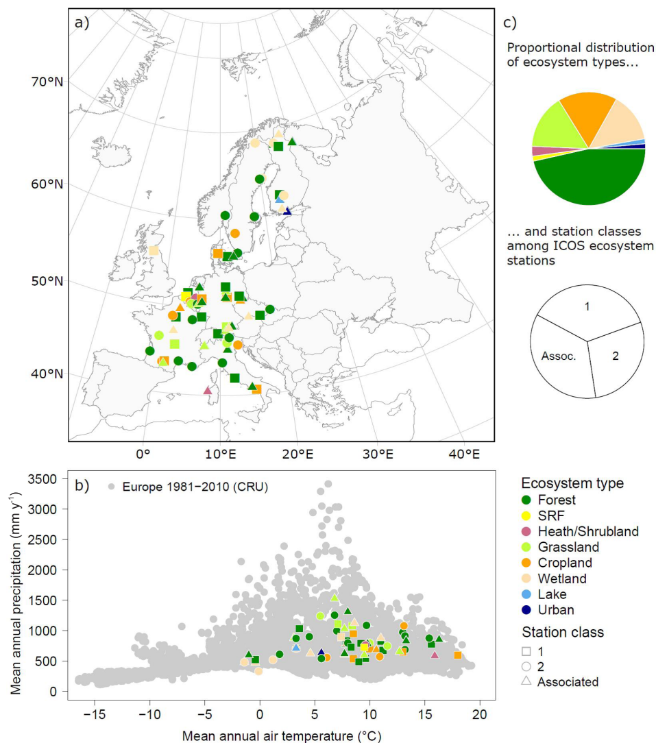
Fig. 2. Overview of ICOS ecosystem stations (Candidate stations and stations with approved label) as of January 2018. Colours indicate the ecosystem types (SRF = Short rotation forestry), and shapes the station classes (see lower panel legend). Stations in Greenland and French Guiana are not included here. a) Spatial distribution of stations on the European continent. Data sources: ArcGis, 2012 (European continent); NOAA, 2016 (Coastlines and European countries). b) Climatological distribution of stations with regard to MAT and MAP (note that averaging periods for both MAT and MAP vary for the different stations) in comparison to MAT and MAP for the reference period 1981–2010 on the European continent for 0.5° grid cells (filled grey circles). Data sources: ArcGis, 2012 (European continent); University of East Anglia Climatic Research Unit (CRU TS4.01). c) Proportional distribution of ecosystem types and station classes among the stations.
