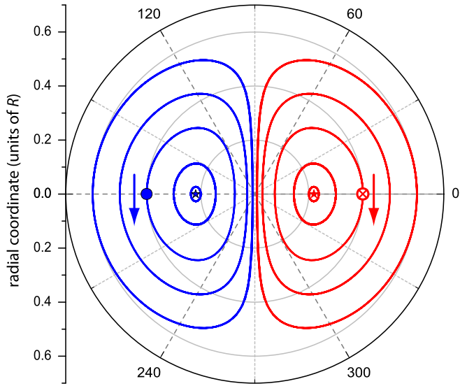
Fig. 2. (Color online.) Typical computed orbits associated with symmetric vortex configurations, determined by integrating the equations of motion [Eqs. (14)]. The vortex on the left (blue) has a counter-clockwise sense of circulation; the vortex on the right (red) has a clockwise sense of circulation. The stationary equilibrium positions of the vortices are indicated by stars. These orbits arise through competition between the effects of interaction and precession [15].
