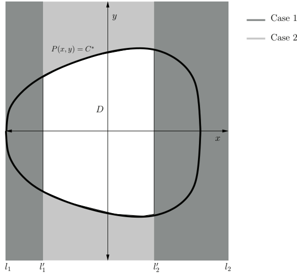
Figure 1: The white region D is positively invariant for system (5)
