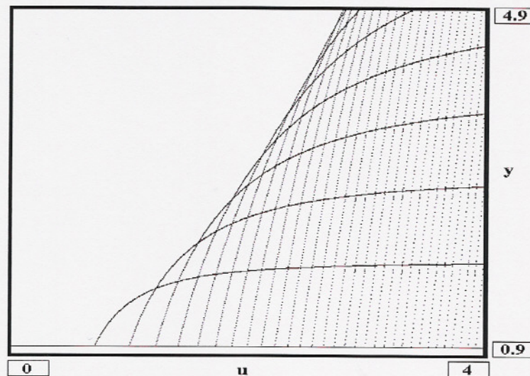
Figure 8: Bifurcation diagram for e = 0.001 .
