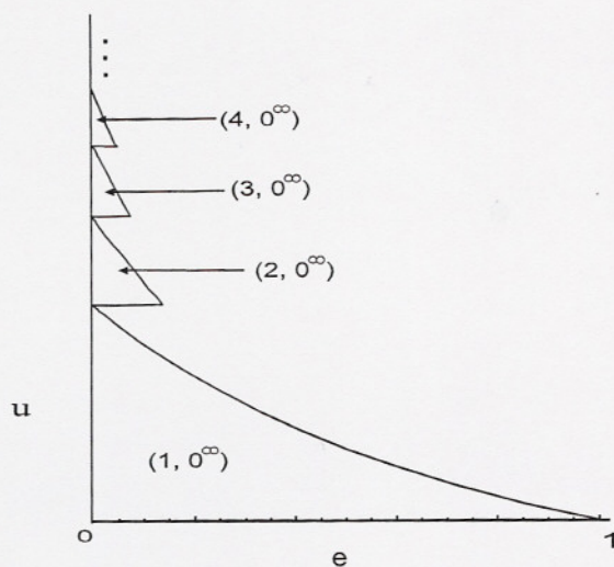
Figure 3: The (n, 0^\infty) -sliding tongues.
