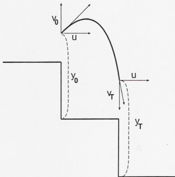
Figure 2: The Poincaré map
