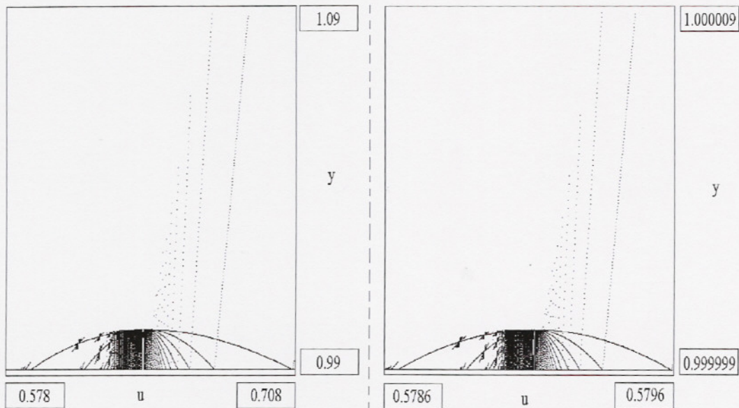
Figure 9: Bifurcation diagrams for e = 0.1 .
