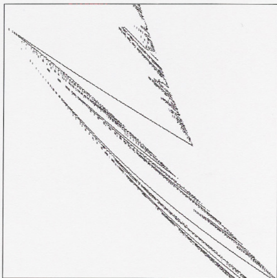
Figure 6: Border of the region [0, 0.333] \times [0.4, 0.733] and the associated box-counting computation.
