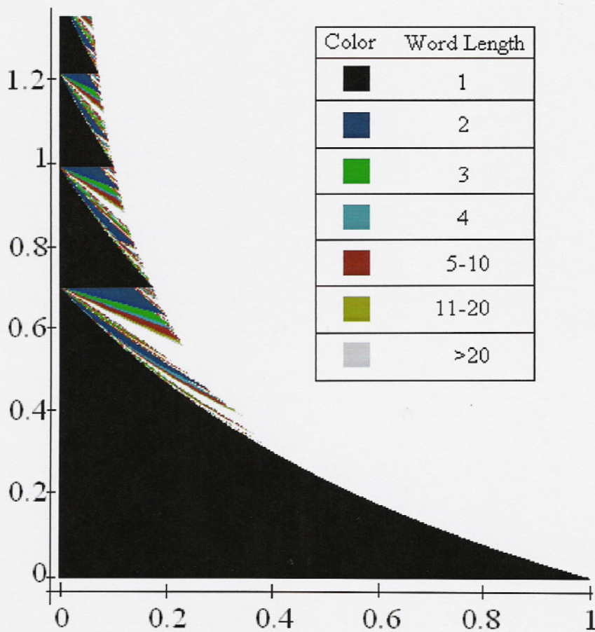
Figure 4: The fractal pattern in the parameter plane e - u .
