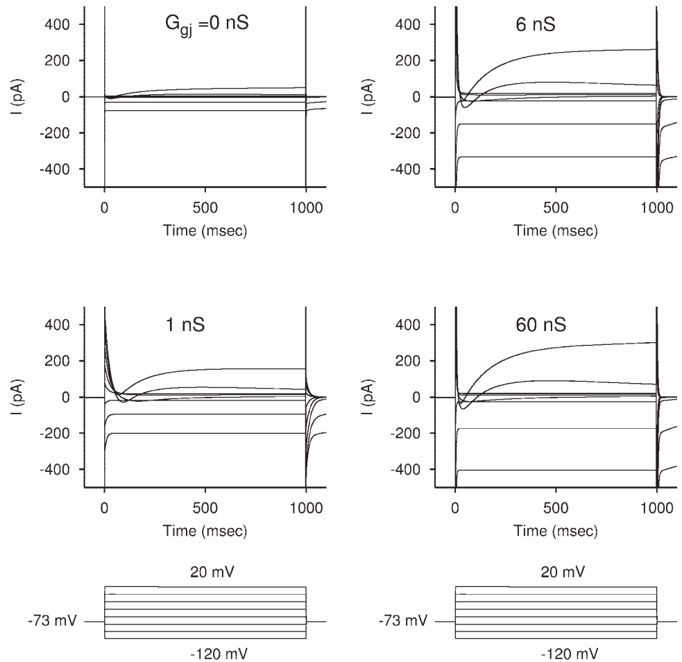
Fig. 3. Voltage-clamp experiments in a cluster of 7 NRK model cells for different degrees of gap junctional coupling ( G_{gj} ) of 0, 1, 6, and 60 nS, as indicated. Buffer parameters were T_B = 20 \mu\text{M} , k_{on} = 320 \text{ mM}^{-1} \cdot \text{s}^{-1} , and k_{off} = 0.06 \text{ s}^{-1} . Series conductance G_{ser} = 50 \text{ nS} (series resistance R_{ser} = 20 \text{ M}\Omega ). Other parameter values are as defined in APPENDIX. Applied voltage step protocols are shown at bottom.
