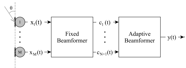
Fig. 1. Schematic implementation of an ADMA. M ... number of microphones, N ... Order of the DMA. c_n(t) ... output signal of fixed beamformer.
