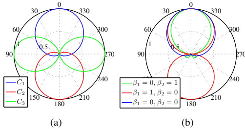
Fig. 3. Beam patterns of the second-order ADMA: (a) Fixed beamformer outputs; (b) Beamformer output for different values of \beta .
