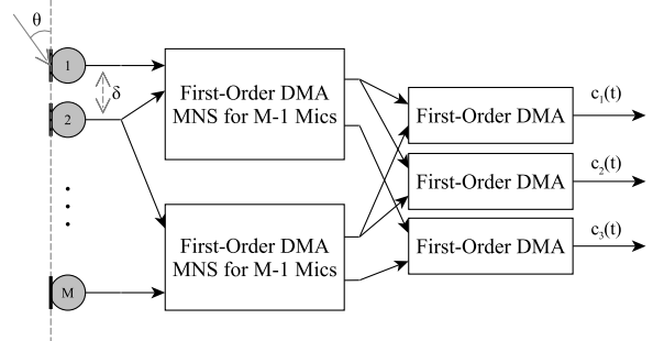
Fig. 5. Schematic implementation of the novel fixed beamformer of a second-order ADMA with the minimum-norm solution.
