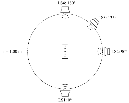
Fig. 6. Recording setup.
