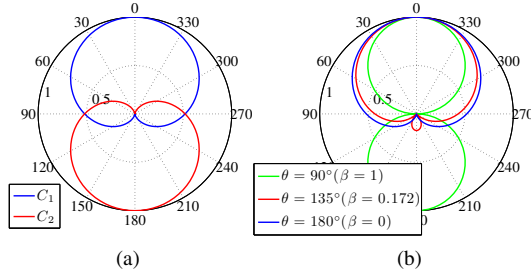
Fig. 2. Beam patterns of the first-order ADMA: (a) Fixed beamformer outputs; (b) Beamformer output for different values of \beta .
