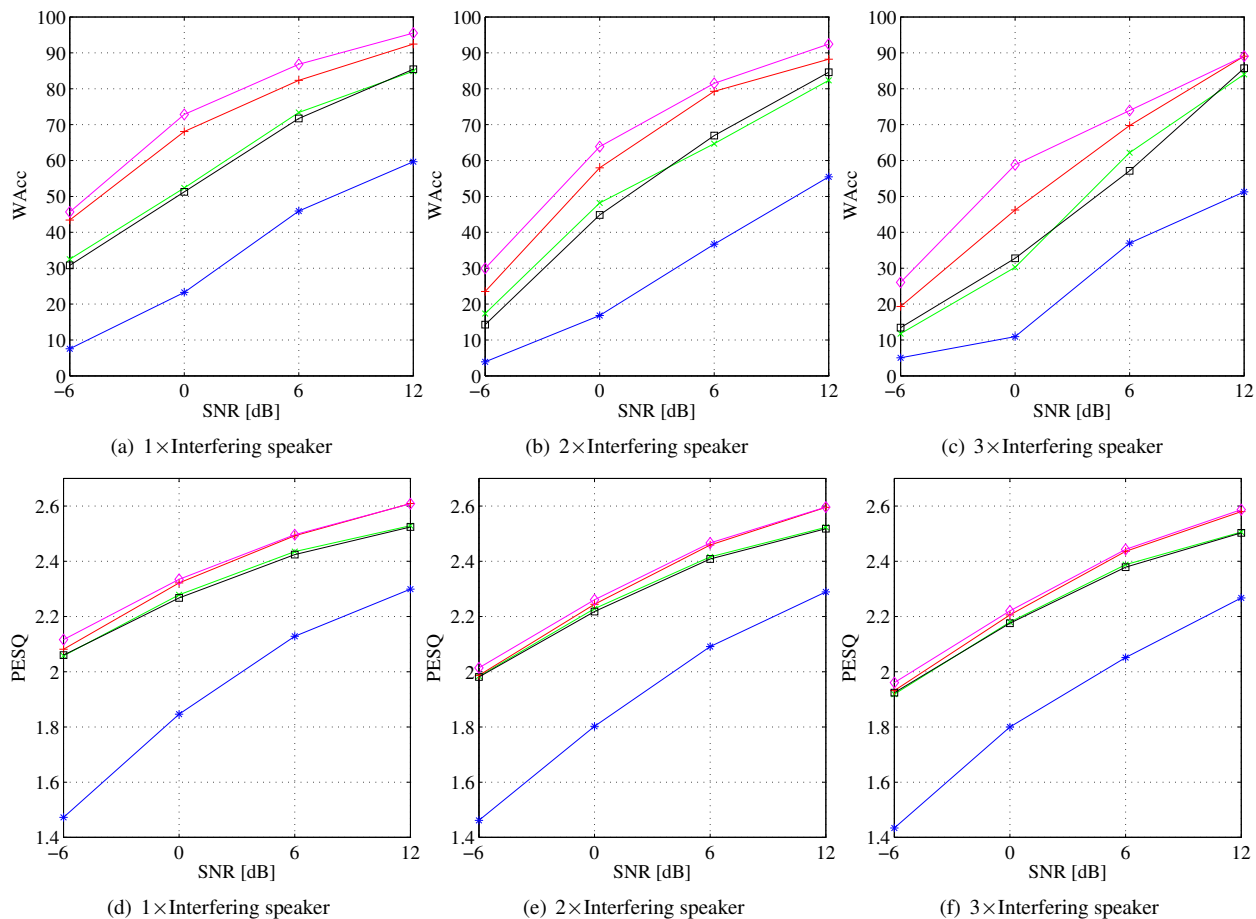
Fig. 7. Results for different scenarios and SNR values: (a - c) WAcc, (d - f) PESQ.
