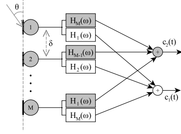
Fig. 4. Schematic implementation of the novel fixed beamformer of a first-order ADMA with the minimum-norm solution.
