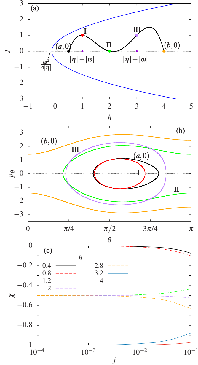
FIG. 9. For the modified spherical pendulum with \omega = -1 and \eta = -2 , (a) the energy momentum plane \mathcal{EM} and tori I=(1, 1), II=(2, 0) and III=(3, 1) (full points) along a path connecting (a, 0) = (0.5, 0) and (b, 0) = (4, 0) , (b) projections of the tori on the plane (\theta, p_\theta) , and (c) \chi(h, j) as a function of j for several values of h .
