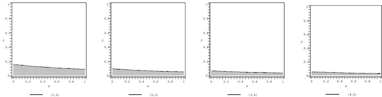
Figure 8.1: The regions of existence (white) of orbits with jump number sequence (1, 2) , (2, 3) , (3, 4) , and (4, 5) , respectively ( x \equiv e_t and y \equiv e_n ).
