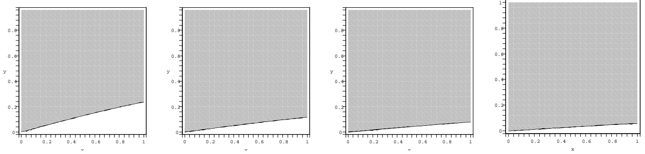
Figure 6.6: The regions of existence (white) of orbits with jump number sequence (02), (03), (04), and (05), respectively ( x \equiv e_t and y \equiv e_n ).
