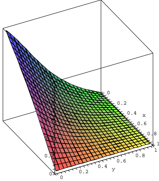
Figure 6.3: The function \kappa_{(0011)} on the unit square, plotted using MAPLE.
